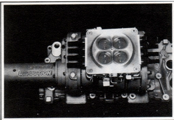
750 HP capabilities from one blower plate.
