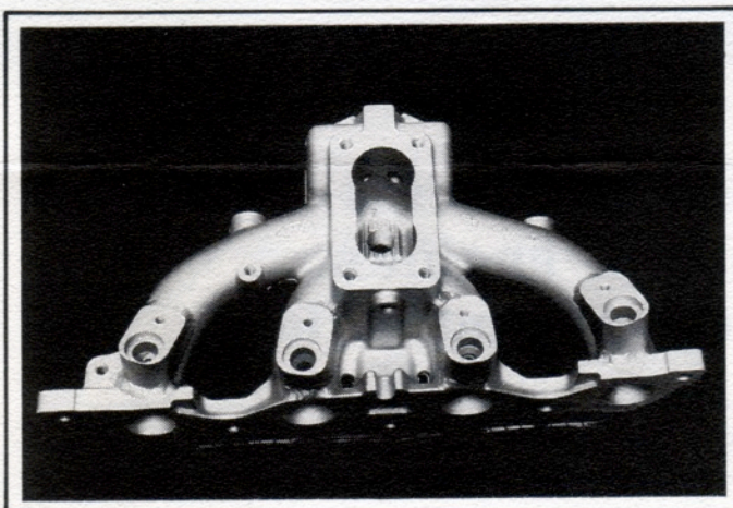
Typical 4 cyl. Injector Placement
