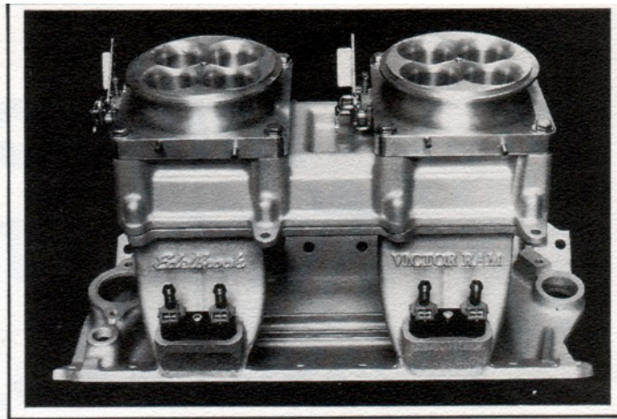
Port injection eliminates the undesirable characteristics of tunnel rams used on street cars.
